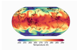
[AMIP (w/o EDMF and topography) simulation.]
