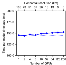
Weak scaling study
