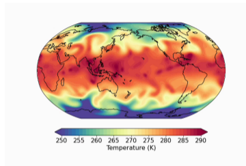
Preliminary AMIP (w/o EDMF and topography) simulation—temperature.
