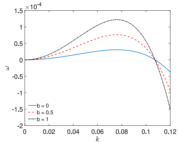
Fig. 4. Growth rate of viscoelastic thin liquid films plotted for surfactant concentration, C = 1 , Contact angle, \theta = 45^\circ , Marangoni number, M = 0.25 and dimensionless interfacial tension, \Sigma_0 = 3 showing the effects of increasing values of slip coefficient, b = 0 (blue solid line), 0.5 (red dashed lines), 1 (black dotted lines). Increasing b leads to an increase in maximum growth rate and hence to a decrease of the rupture time.
